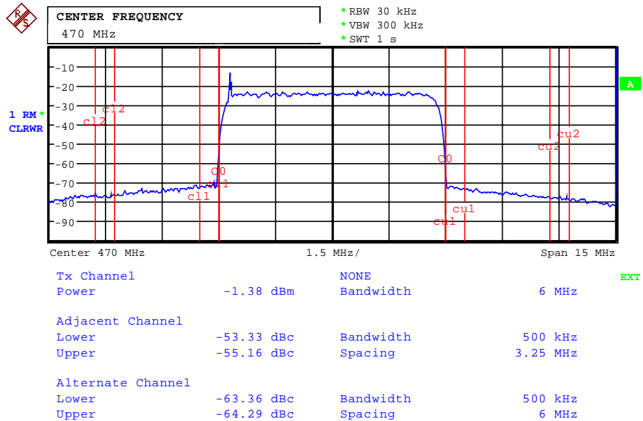
Fig. 6 FSP screen with ACP measurement to FCC Regulation 47CFR 73.622 The ACP measurement settings to FCC Regulation 47CFR 73.622 are:
